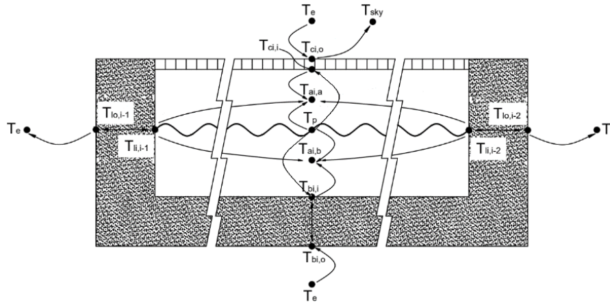
Fig. 2. Scheme of temperature nodes and thermal transmission circuits.
