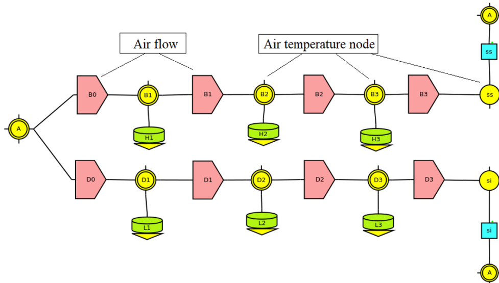
Fig. 3. Model representation of air mass flow through the collector. B0-3 and D0-3 correspond to the air flow above and below the absorber plate, respectively.
