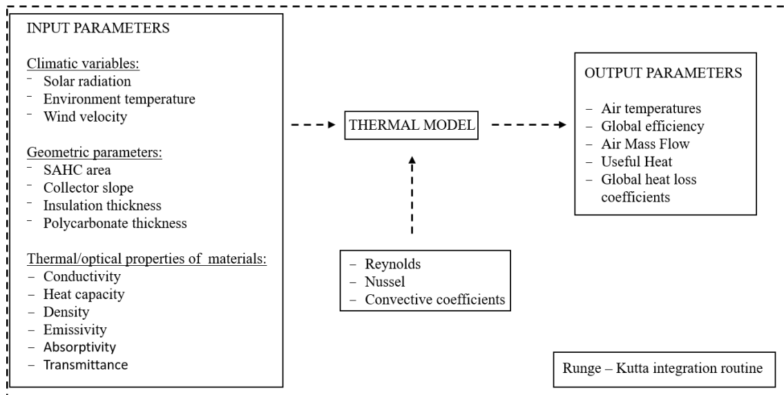
Fig. 5. Scheme of the thermal model implemented on Simusol.
