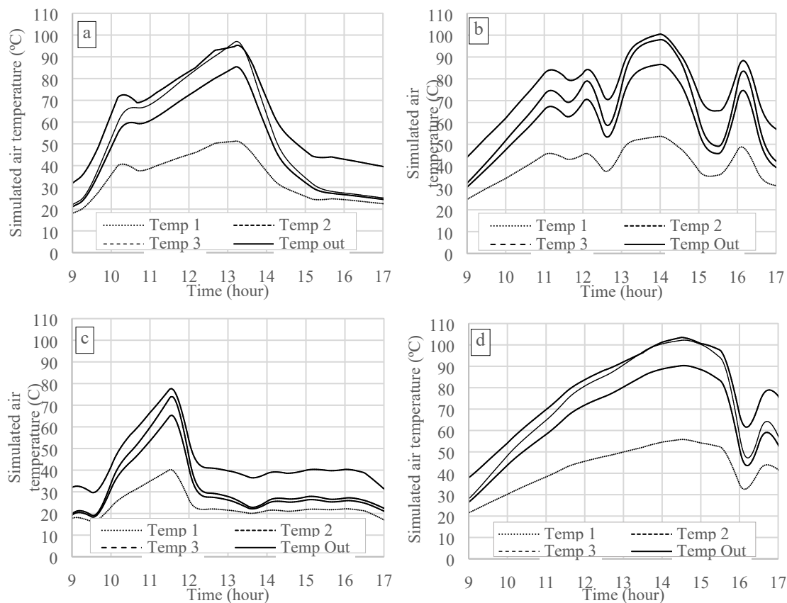
Fig. 6. Simulated air temperature for the upper channel. Temp 1 to 3, and Temp out correspond to nodes B 1 to 3 and temp ss in Fig. 3. a) March 29, b) April 6, c) April 12, d) April 15.
