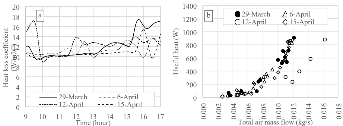
Fig. 9. a) Global heat loss coefficients. b) Useful heat gain related to the total air mass flow.
