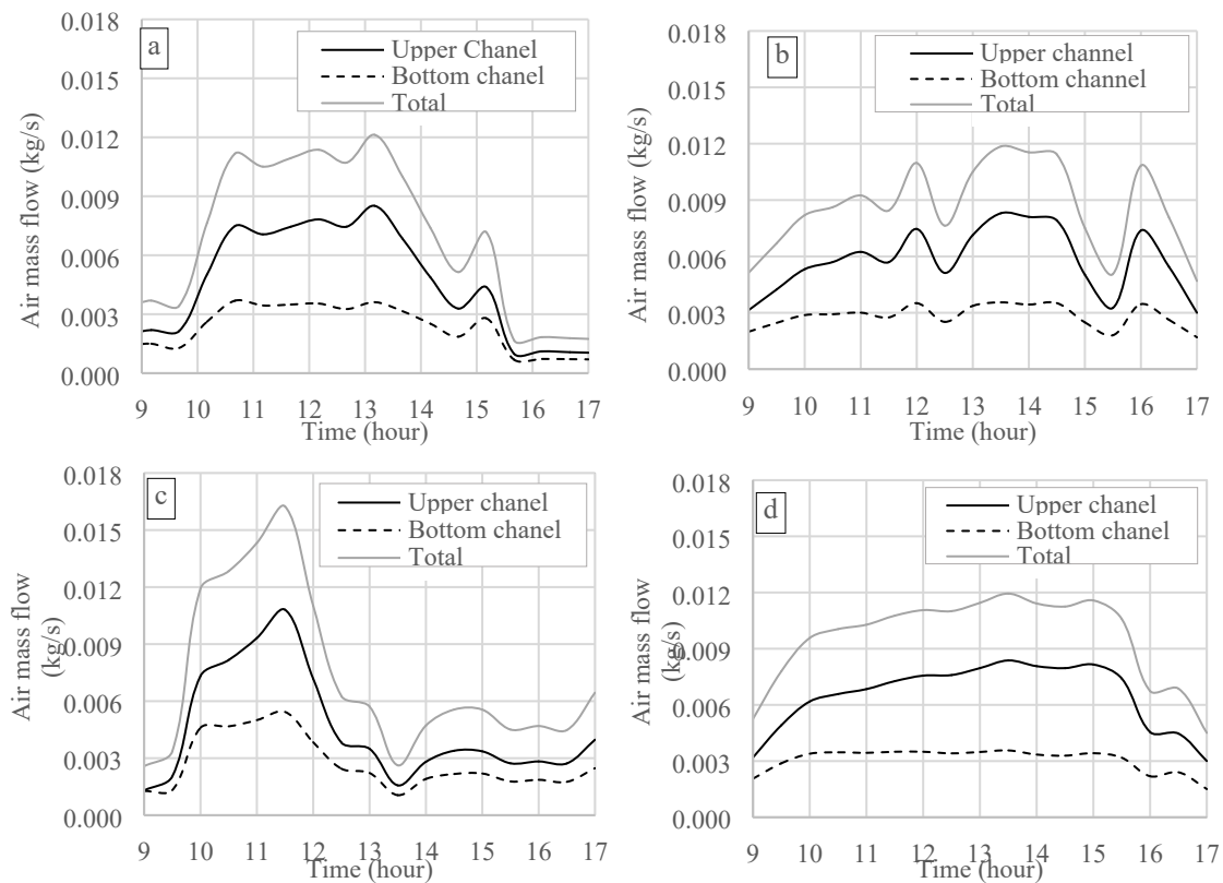
Fig. 7. Air mass flow profiles for both upper and bottom channels of the SAHC and total air mass flow. a) March 29, b) April 6, c) April 12, d) April 15.
