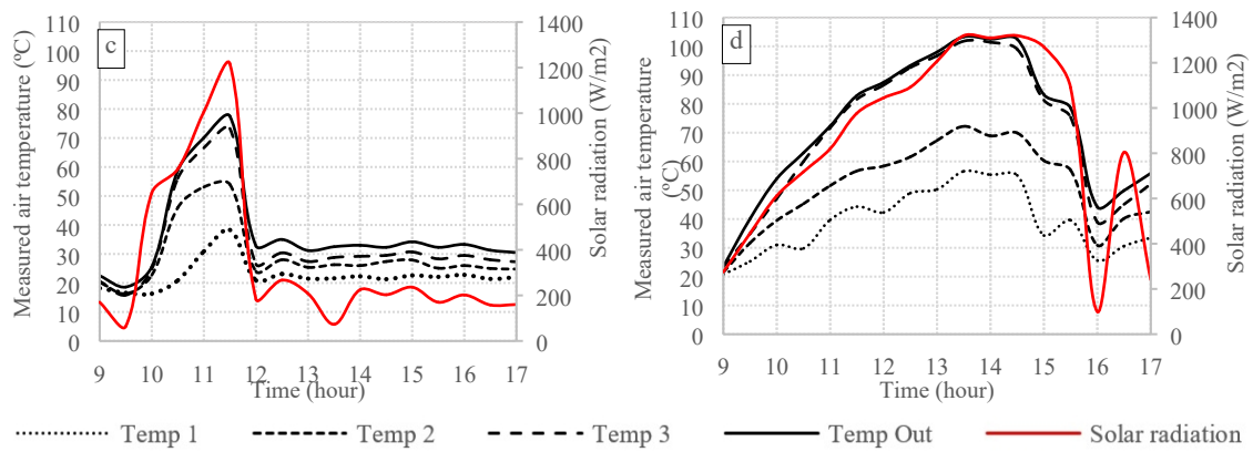
Fig. 10. Measured air temperatures in the upper channel. The Temp out plot corresponds to the ss node from the simulation. a) March 29, b) April 6, c) April 12, d) April 15.
