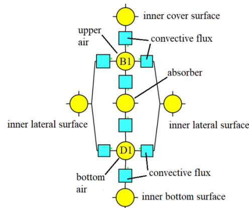
Fig. 4. Scheme of convective fluxes into air flow nodes, for the first section of the SAHC.
