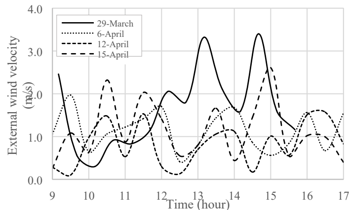
Fig. 12. External wind velocity surrounding the SAHC.
