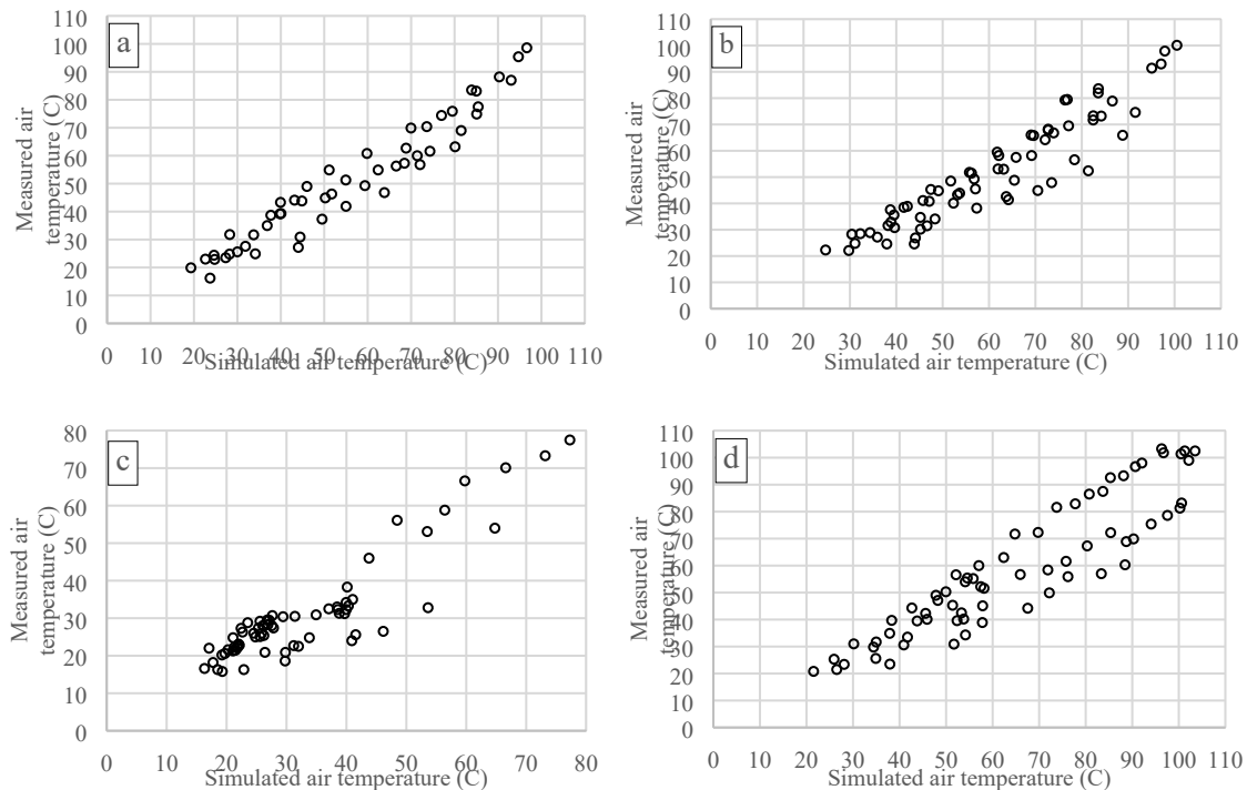
Fig. 11. Comparison between experimental and numerical air temperatures. a) March 29, b) April 6, c) April 12, d) April 15.
