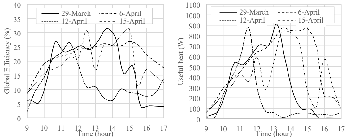
Fig. 8. Global efficiency (a) and useful heat gain (b).
